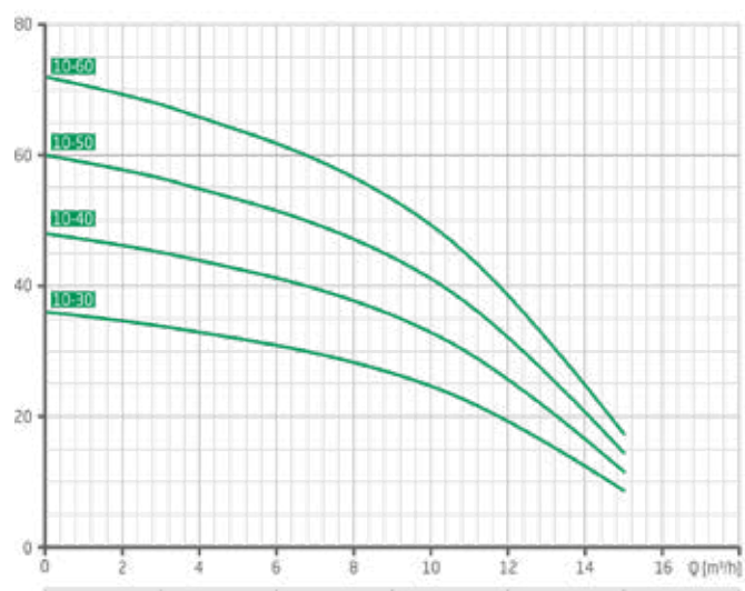
Characteristics MTX 10
