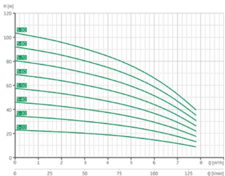
Characteristics MTX 5
