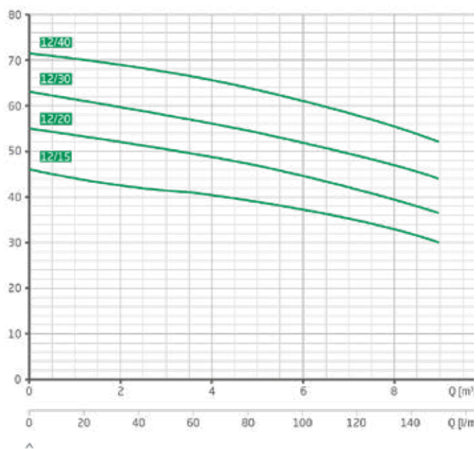
Characteristics 2 VGX 12
