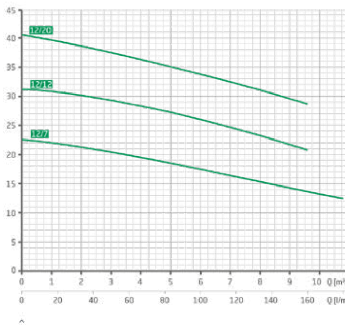
Characteristics VGX 12
