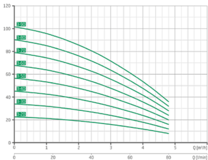
Characteristics MTX 3
