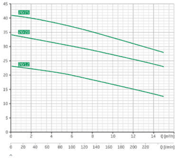
Characteristics VGX 20
