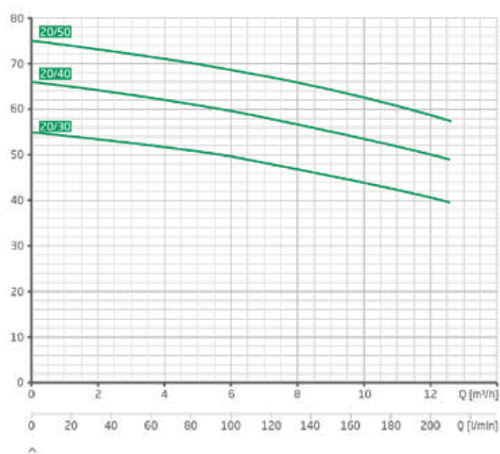
Characteristics 2 VGX 20
