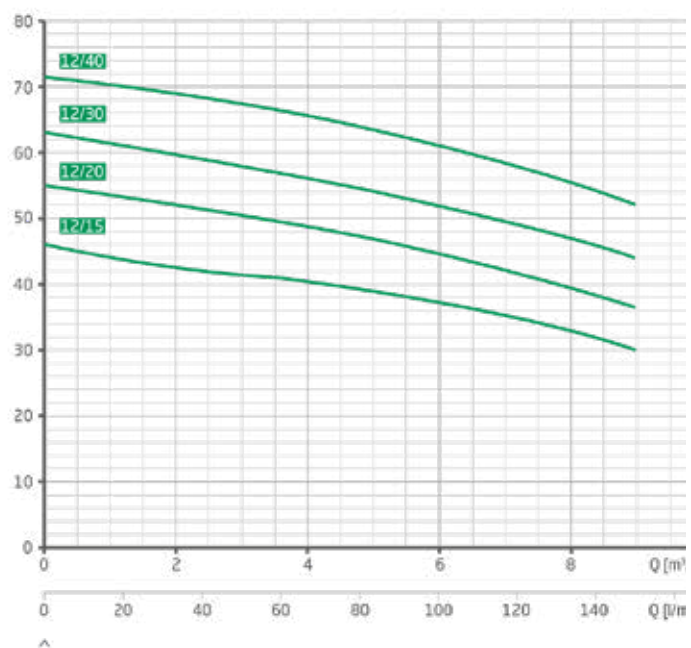
Characteristics 2 VGX 12
