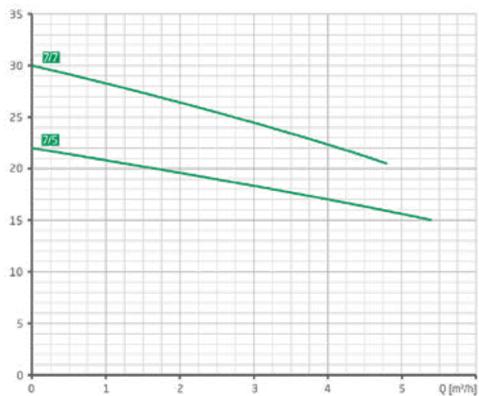
Characteristics VGX 7
