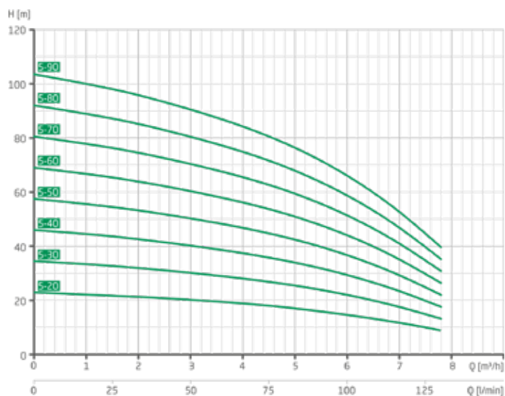
Characteristics MTX 5
