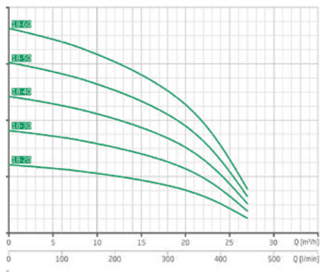
Characteristics MTX 18
