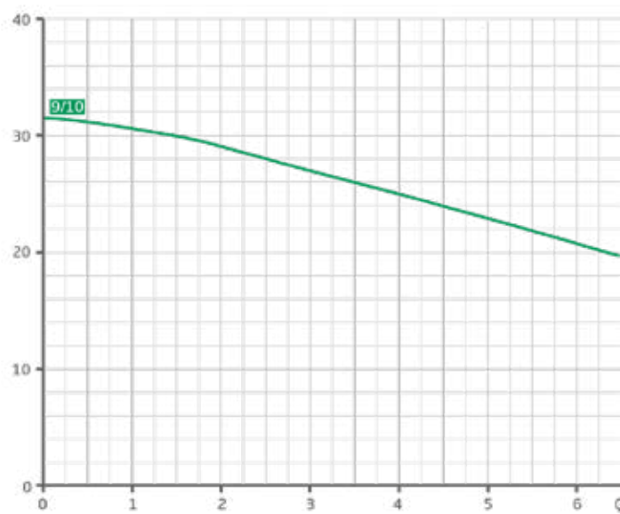
Characteristics VGX 9
