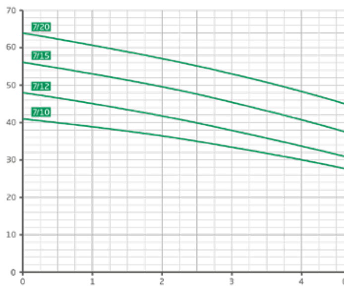
Characteristics 2 VGX 7
