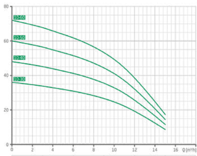
Characteristics MTX 10
